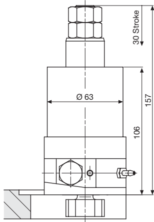
Tie rod retracted Swivelling angle 0°
