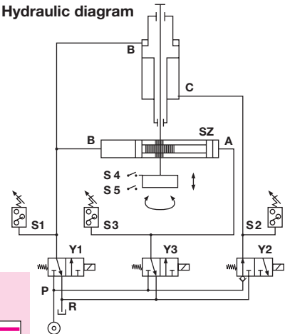
Hydraulic diagram
