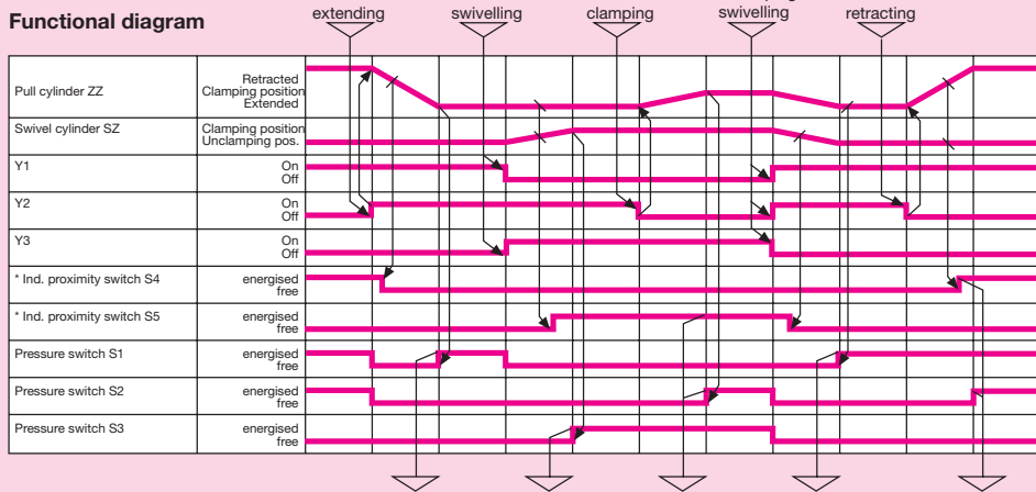
Functional diagram
