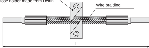
Part-no. 5.5065.0003 Hose holder made from Delrin
