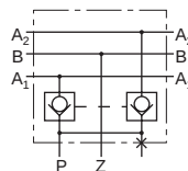
Schematic symbol
