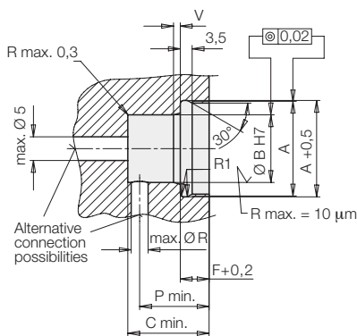
Manifold-mounting hole
