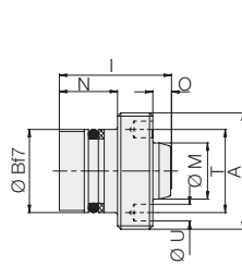
Threaded nipple
