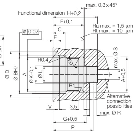
Manifold-mounting hole
