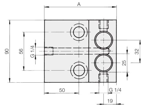
Locking force 100 bar [kN] 9.8 at 500 bar [kN] 49.0 Piston stroke, max. [mm] 2
