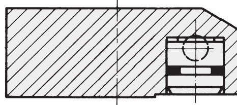
Locking force 100 bar [kN] >4.9 at 500 bar [kN] 24.5 Piston stroke, max. [mm] 2
